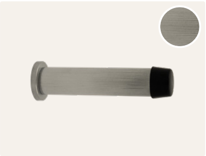
5292 Solid Brass – Linear Knurl 85mm x 25mm Slimline Base STOCKED SIGNATURE BLK, BN , CCB, GN, MSB DRB, RB, RLB, OR, USB
