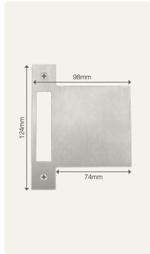
1165 - Maximum length only shown please specify length required upon ordering. STOCKED SIGNATURE SS AB, DRB, MSB, NB, OR, PB, PC, RB, RLB, UB, USB
