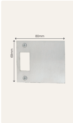
1163 - Maximum length only shown please specify length required upon ordering. STOCKED SIGNATURE SS AB, DRB, MSB, NB, OR, PB, PC, RB, RLB, UB, USB
