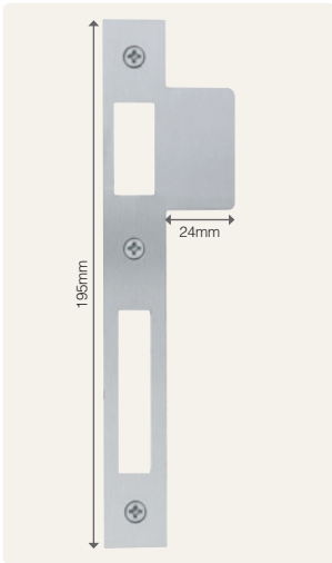
1234 LH (pic) or RH - Maximum length only shown please specify length required upon ordering. STOCKED SIGNATURE SS PC
