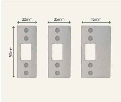
1451 32mm (left pic) 1452 35mm (middle pic) 1453 45mm (right pic) - To go over existing Windsor standard latch cropping STOCKED SIGNATURE SS AB, DRB, MSB, NB, OR, PB, PC, RB, RLB, UB, USB
