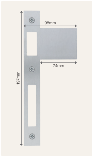
1187 LH (pic) or RH - Maximum length only shown please specify length required upon ordering.
