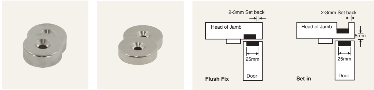
MAGNET INSTALLATION DIAGRAM
