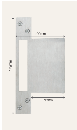
1164 - Maximum length only shown please specify length required upon ordering. STOCKED SIGNATURE SS AB, DRB, MSB, NB, OR, PB, PC, RB, RLB, UB, USB
