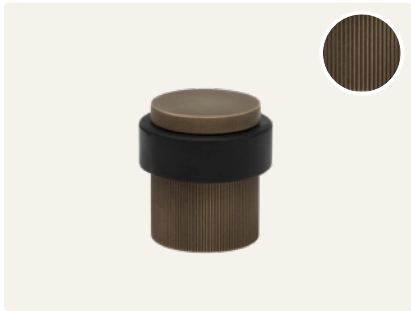
5294 Solid Brass – Linear Knurl 38mm x 30mm STOCKED SIGNATURE BLK, BN, CCB, GN, MSB DRB, RB , RLB, OR, USB
