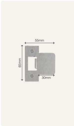
1125 - Maximum length only shown please specify length required upon ordering.
