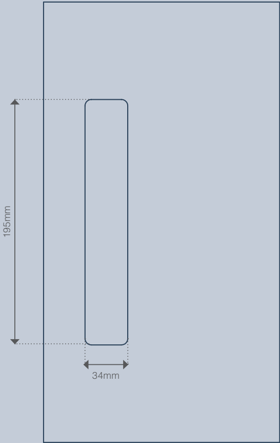
5620 INSTALLATION DIAGRAM
