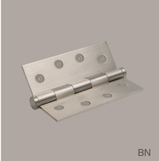
5906 Loose Pin Flat Tip 5902 Fixed Pin Flat Tip (No PC) 100mm x 75mm Solid Brass
