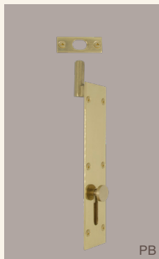
5271 Necked Throw - Inward > 105mm x 31mm > 25mm throw > 20mm offset
